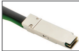
QSFP/QSFP Passive, Madison 28AWG
